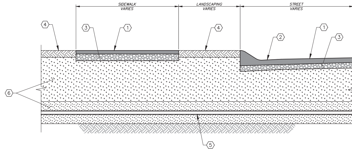
HMAC STREET, CURB, GUTTER, & SIDEWALK PATCH SECTION N.T.S.
