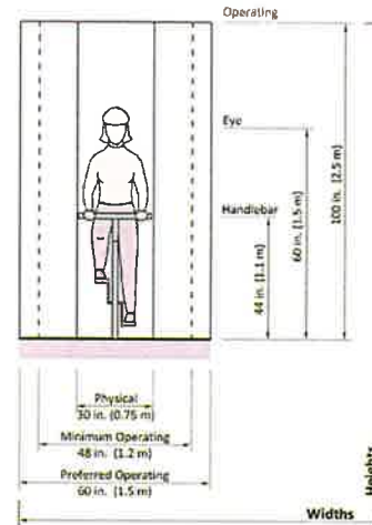
Figure 31. Bicyclist operating space (AASHTO, 2012).
