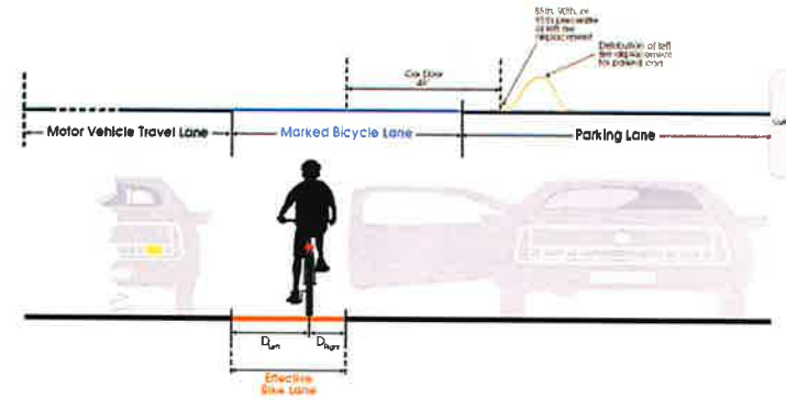
Figure 30. Illustrating the effective bike lane and central positioning.
