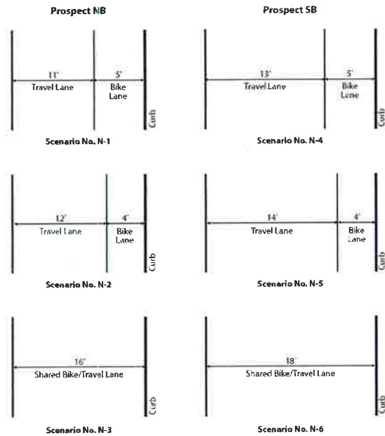
Figure 2. Study sites and scenarios without on-street parking.
