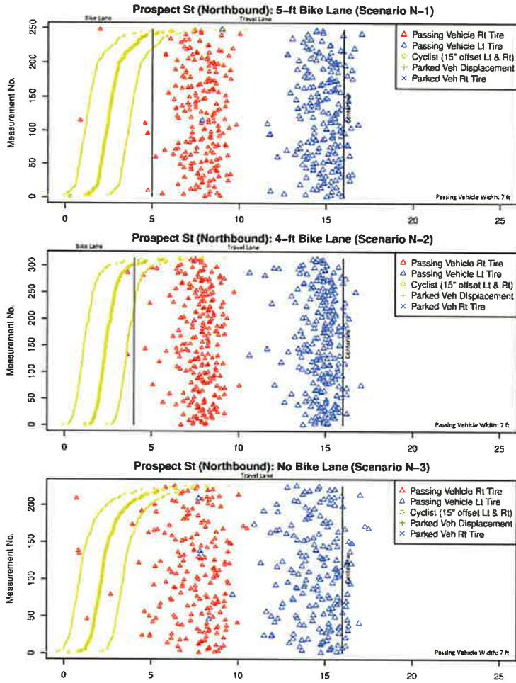
Figure 12. Measurements taken on Prospect Street (northbound) in Cambridge (assumed 7-ft width for passing vehicle).
