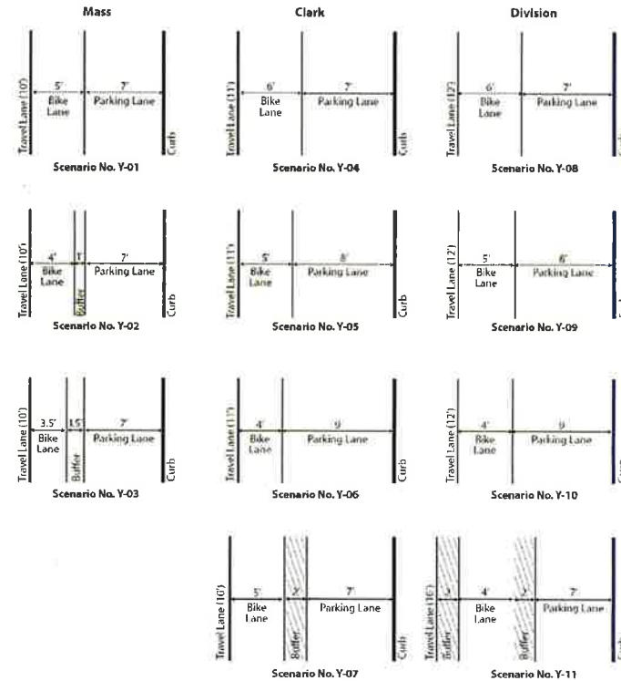
Figure 1. Study sites and scenarios with on-street parking.
